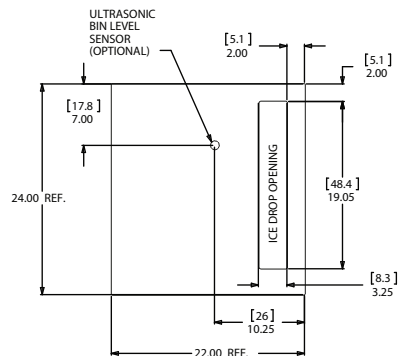
PLAN VIEW
