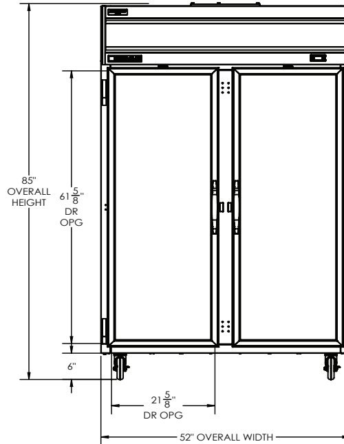
ELEVATION VIEW
