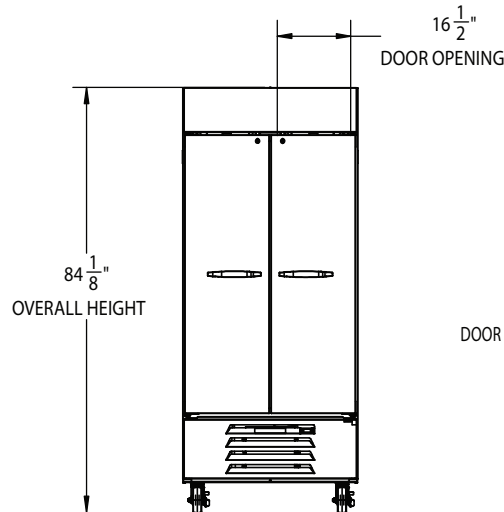
ELEVATION VIEW
