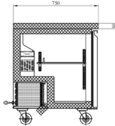
SECTION VIEW
