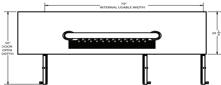
ELEVATION VIEW
