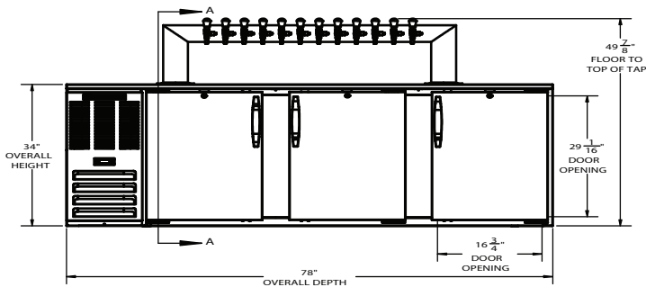
ELEVATION VIEW
