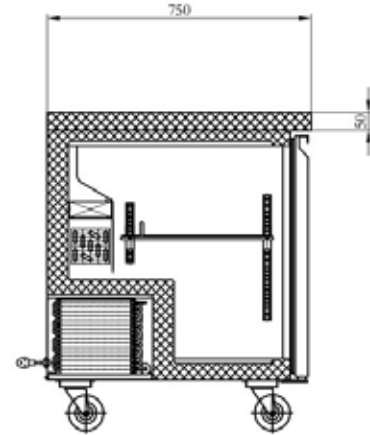
SECTION VIEW
