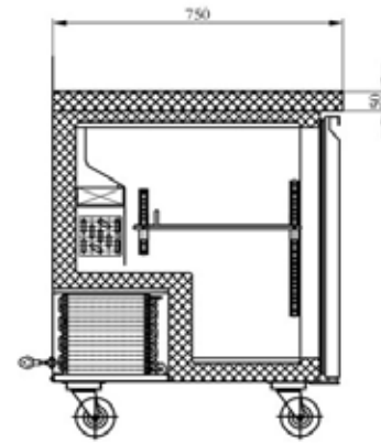
SECTION VIEW
