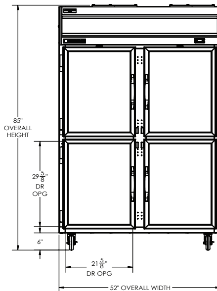
ELEVATION VIEW
