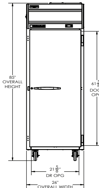
ELEVATION VIEW
