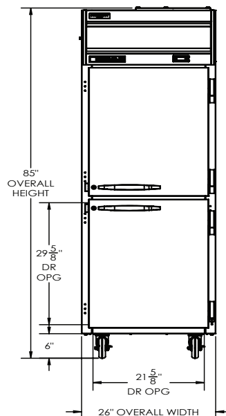
ELEVATION VIEW
