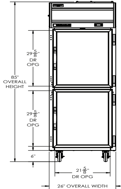
ELEVATION VIEW
