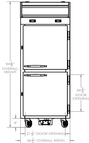
ELEVATION VIEW
