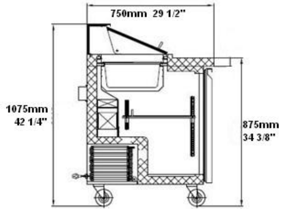
Section View
