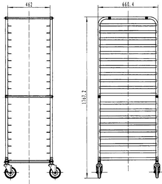
Dimensions for Full Size Bun Pan Rack
