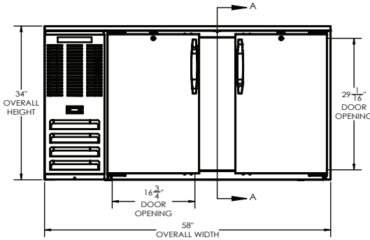
ELEVATION VIEW
