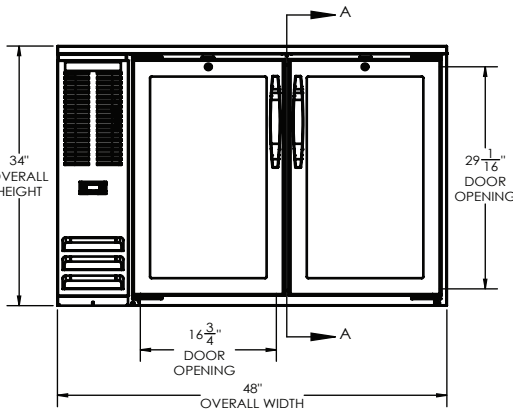
ELEVATION VIEW
