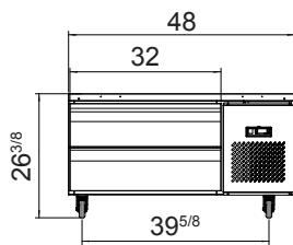
MGF8460GR
