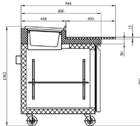
SECTION VIEW
