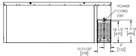
BACK VIEW
