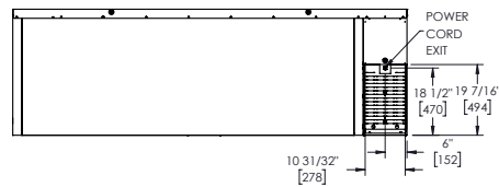
BACK VIEW
